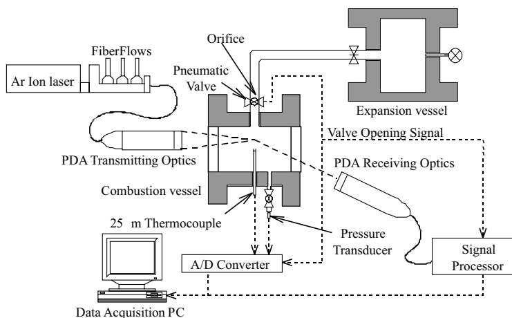
Figure 1. Experimental apparatus for droplet size measurement using Phase Doppler Anemometry (PDA) system.
