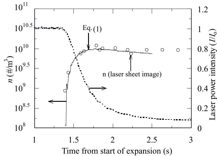
Figure 5. Variation with time of laser power attenuation and droplet number density. Conditions are the same as in Figure 3.
