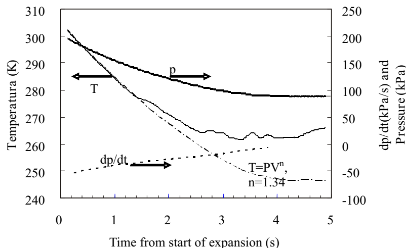
Figure 3. Variation of pressure and temperature with time after the start of expansion of a stoichiometric mixture of iso-octane-air. The initial conditions were 200 kPa and 303 K.
