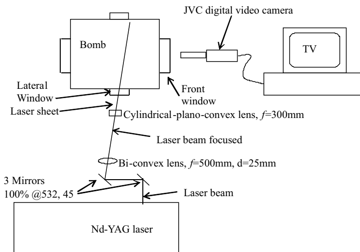
Figure 2. Apparatus arrangement of laser sheet imaging for n estimation.
