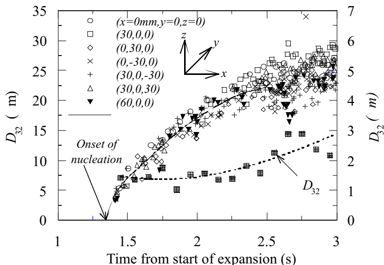
Figure 4. Droplet size variation with time and space. Conditions are the same as in Figure 3.
