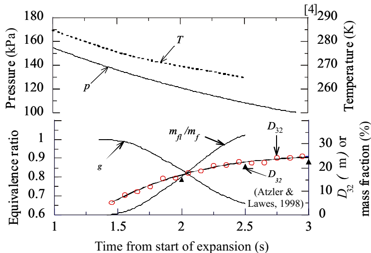
Figure 6. Variation of all relevant mixture properties with time during expansion. Conditions are the same as in Figure 3.
