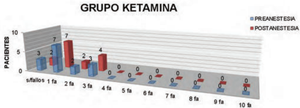
Fig. 2. SPMSQ (PFEIFFER).
