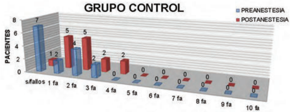
Fig. 1. SPMSQ (PFEIFFER).
