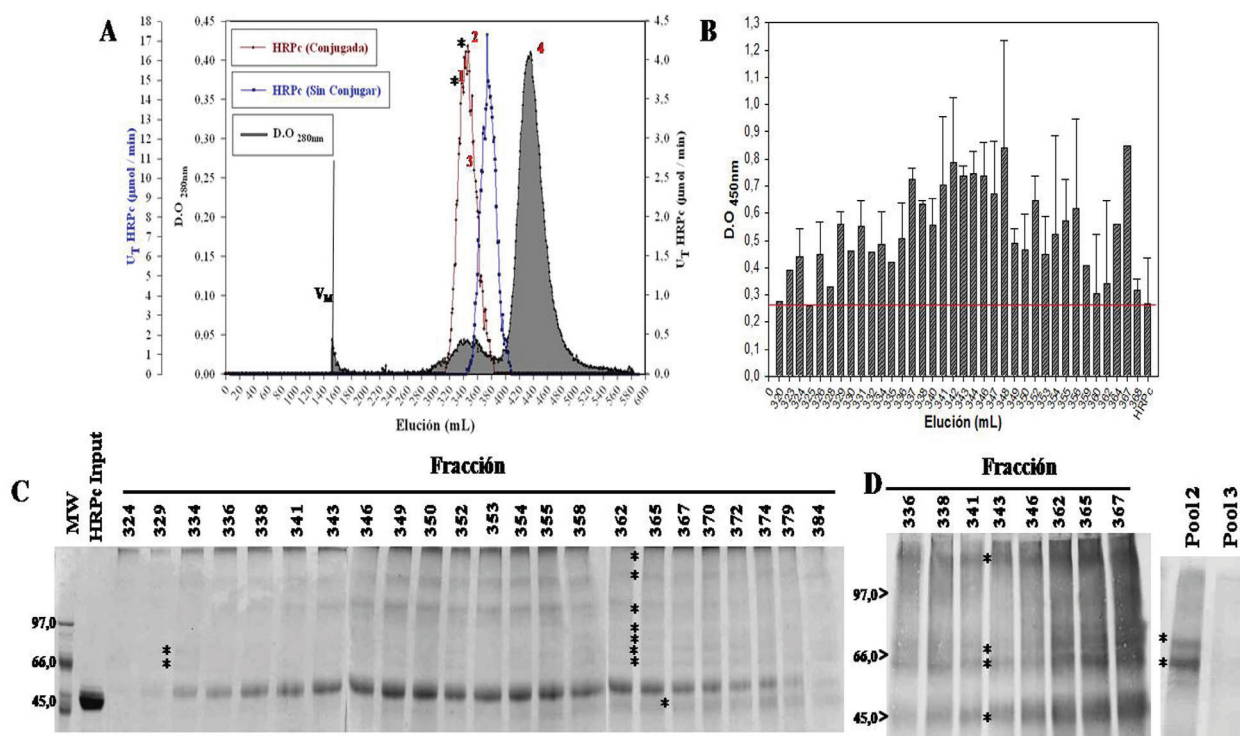
Fig. 3. A) Elution profile consensus at 280 nm and 414 nm corresponding to the separation of HRPc-rK346 conjugates by SEC (Sephacryl S-200). Conjugation was performed with GA 1.25%. Profiles at 414 nm shown in red and blue correspond to the determination of EA of the conjugated and non-conjugated HRPc respectively. Asterisks indicate the two peaks with HRPc activity measured at 414 nm (1 and 2). Maximal absorbance at 280 nm (3 and 4) were also determined. B) Direct ELISA corresponding to fractions with the greatest conjugated-HRPc activity. The SD for two replicates is shown as well as the basal detection limit (red line). C) Visualization of HRPc-rK346 conjugates by SDS-PAGE at 10% and D) by Western-blot. Each lane in Fig. C shows those fractions evaluated by direct ELISA, corresponding to the peak with conjugated-HRPc activity. Conjugates are indicated by asterisks. Pool 2: Fractions with the most HRPc activity (323-388 mL of elution). Pool 3: (413-452 mL of elution).
