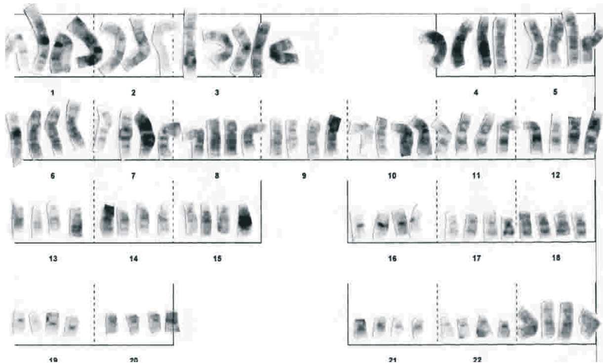
Fig. 2. Karyotype with polyploidy: 92,XXXX.
