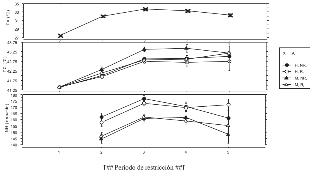
FIGURA 2. VARIACIONES DE LA TEMPERATURA CORPORAL (TC) Y NIVEL DE HIPERVENTILACIÓN (NH), SEGÚN CAMBIOS DE LA TEMPERATURA AMBIENTE (TA) A LO LARGO DE EXPERIENCIA 1 ( EXP 1) Y EXPERIENCIA 2 (EXP 2) DURANTE LOS DIFERENTES PERIODOS DEL DÍA (EXP. 1 2=6:30 A 8:00 3 = 10:30 A 12:00 4= 13:30 A 15:00 5= 17.00 A 18:30) Y (EXP. 2 1=7:30 A 9:00 ; 2= 10:30 A 12:00; 3=14:00 A 15:30; 4=17:00 A 18:30; 5=19:00 A 20:30), SEGÚN TRATAMIENTO DE RESTRICCIÓN DE ALIMENTO (NR = NO RESTRINGIDO Y R = RESTRINGIDO) Y SEXO DE LOS POLLOS (H= HEMBRA Y M = MACHO)/ VARIATIONS OF THE CORPORAL TEMPERATURE (TC) AND LEVEL OF HIPERVENTILACIÓN (NH), ACCORDING TO CHANGES OF THE TEMPERATURE ENVIRONMENT (TA) ALONG EXPERIENCE 1 (EXP 1) AND EXPERIENCE 2 (EXP 2) DURING THE DIFFERENT PERIODS OF THE DAY (EXP. 1 2=6:30 To 8:00 3 = 10:30 To 12:00 4 = 13:30 To 15:00 5 = 17.00 To 18:30) And (EXP. 2 1=7:30 To 9:00; 2 = 10:30 To 12:00; 3=14:00 To 15:30; 4=17:00 To 18:30; 5=19:00 To 20:30), ACCORDING TO TREATMENT OF FOOD RESTRICTION (NR = NOT RESTRICTED AND R = RESTRICTED) AND SEX OF THE CHICKENS (H = FEMALE AND M = MACHO).
